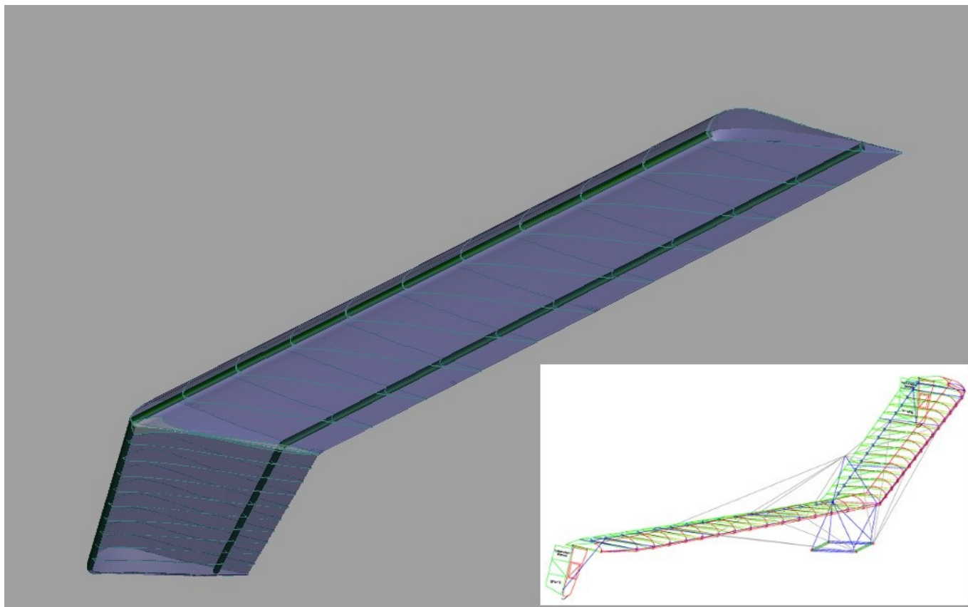
gnu-V rigid wing design. CAD render by Ciel Ouvert
